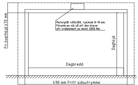
Overmontert motor, standard montering
